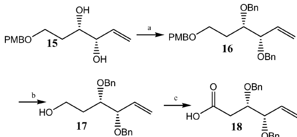
Scheme 4. Synthesis of acid 18 : (a) BnBr, NaH, THF, 0 °C to room temp., 4 h, 85%; (b) DDQ, CH 2 Cl 2 /H 2 O, room temp., 30 min, 93%; (c) (i) IBX, EtOAc, reflux, 3 h; (ii) NaClO 2 , NaH 2 PO 4 , DMSO, overnight, 80%.
