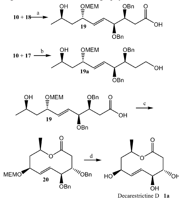
Scheme 5. Synthesis of decarestrictine D through cross-metathesis and Yamaguchi macrolactonization: (a) RuCl 2 (=CHPh)(PCy 3 )-(IEMS), CH 2 Cl 2 , room temp., 2 days, 54%; (b) RuCl 2 (=CHPh)-(PCy 3 )(IEMS), CH 2 Cl 2 , room temp., 2 days, 38%; (c) 2,4,6-trichlorobenzoyl chloride, Et 3 N, THF, 2 h, room temp. then C 6 H 6 , DMAP, 80 °C, 1 h then reflux, 1 h, 32%; (d) TiCl 4 , CH 2 Cl 2 , 0 °C to room temp., 30 min, 78%.
